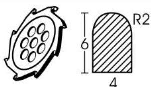
Carbide blade Ø 110 x 4 mm, round
