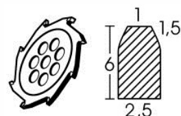
Carbide blade Ø 110 x 2.5 mm
