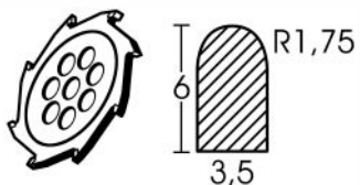
Carbide blade Ø 110 x 3.5 mm, round
