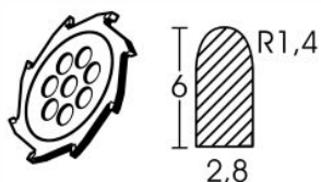
Carbide blade Ø 110 x 2.8 mm, round
